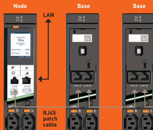
Deployment illustration with one daisy chain on feed A and one daisy chain on feed B
